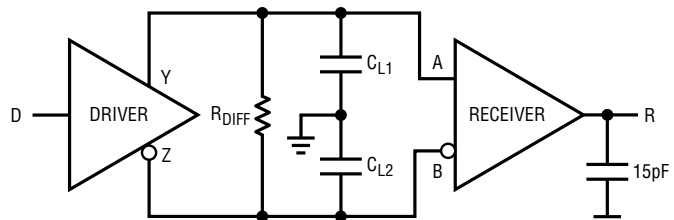
Figure 2. Driver/Receiver Timing Test Circuit
