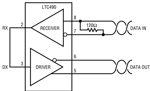
Figure 6. Line Repeater
