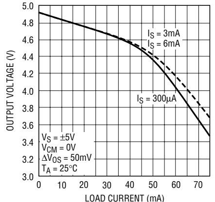
Output Voltage Swing vs I_{\text{LOAD}}
