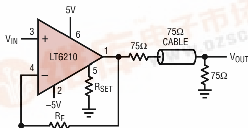
Line Driver Configuration for Various Supply Currents
