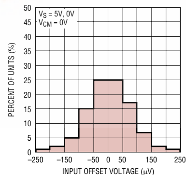
V OS Distribution, V CM = 0V (S8, PNP Stage)
