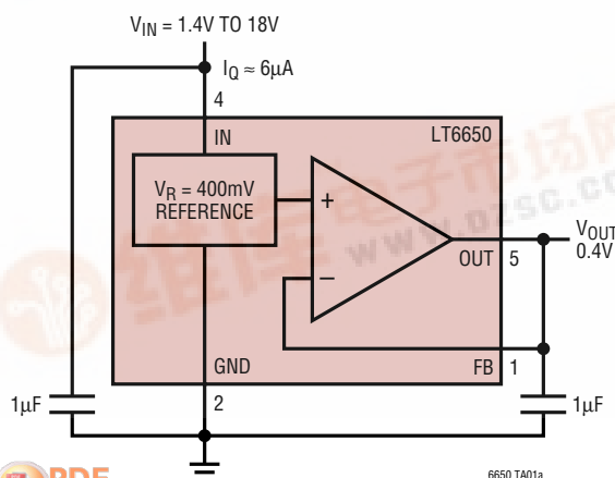
Battery-Powered 0.4V Reference
