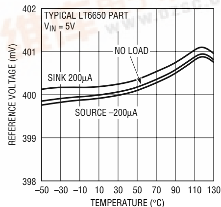
LT6650 Temperature Drift
