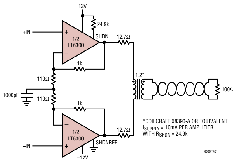
High Efficiency \pm 12V Supply ADSL Line Driver
