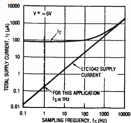
Total Supply Current vs Sampling Frequency
