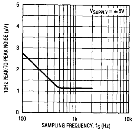
10Hzp-p Noise vs Sampling Frequency
