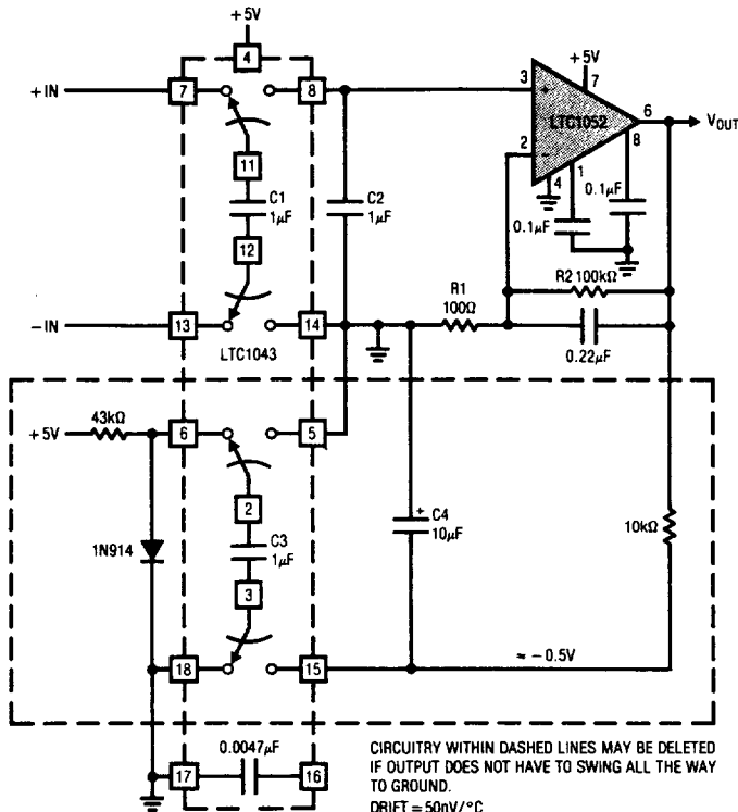
5V Powered Ultra Precision Instrumentation Amplifier
