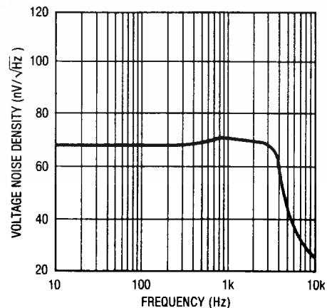
LTC1051 Noise Spectrum
