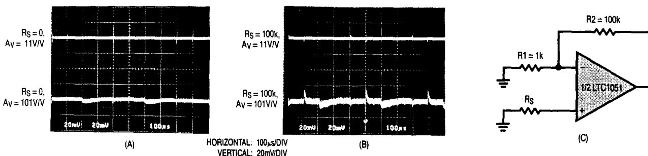
Figure 2. Clock Feedthrough
