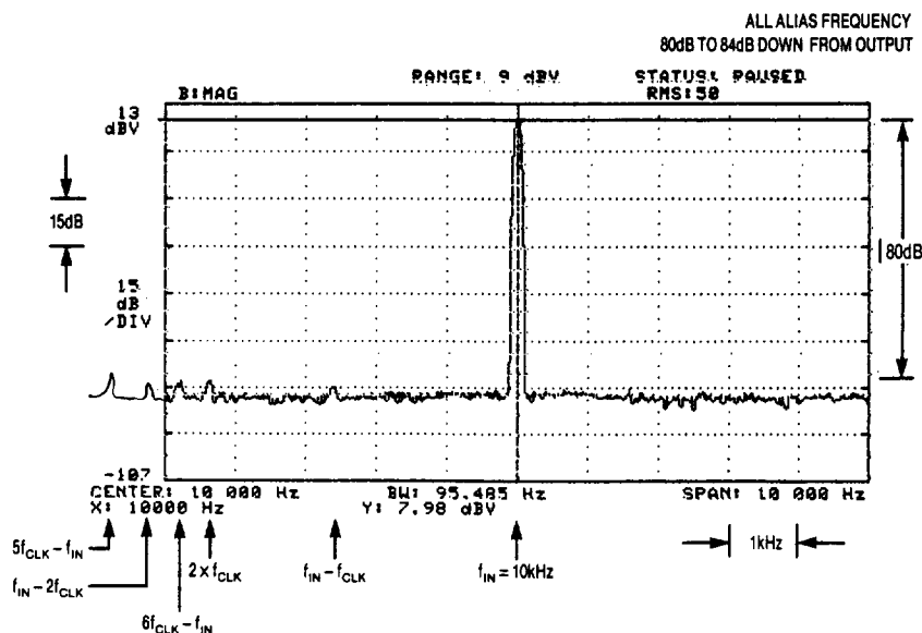
Figure 6B. Output Voltage Spectrum of 1/2 LTC1051, Operating as a Unity Gain Inverting Amplifier. V_S = \pm 5V , R_L = 10k , C_L = 50pF , V_{IN} = 8Vp-p , 10kHz .
