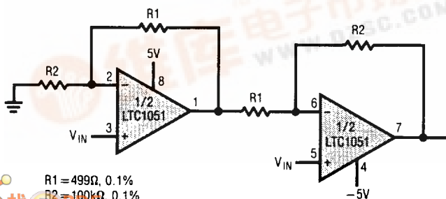
High Performance Low Cost Instrumentation Amplifier
