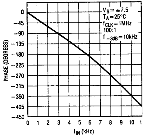
Graph 2. Phase Response
