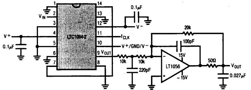
Figure 5. Adding an Output Buffer-Filter to Eliminate Any Clock Feedthrough. Passband \pm 0.1dB to 50kHz, -3dB at 94kHz.
