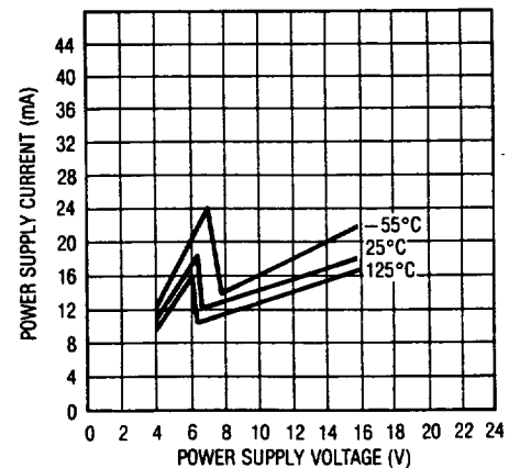
Graph 9. Power Supply vs Current
