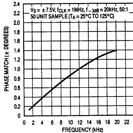
Graph 5. Phase Matching
