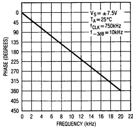
Graph 2. Phase vs Frequency
