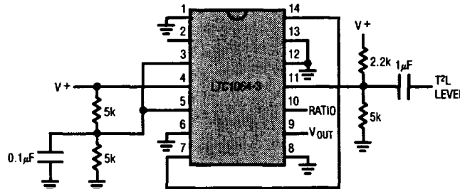
Figure 4. Level Shifting the Input T²L Clock for Single Supply Operation ≥ 6V.
