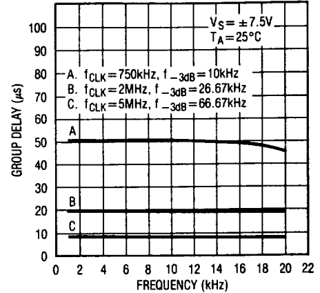
Graph 3. Group Delay
