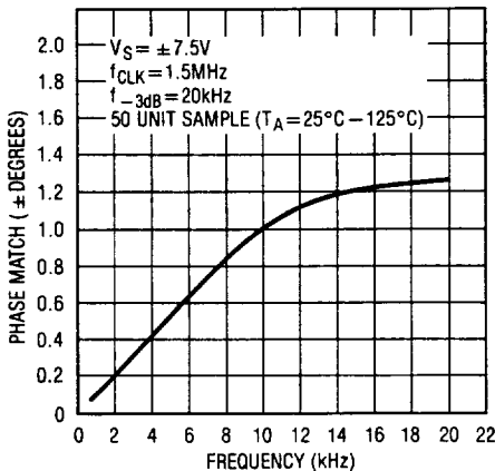
Graph 4. Phase Matching
