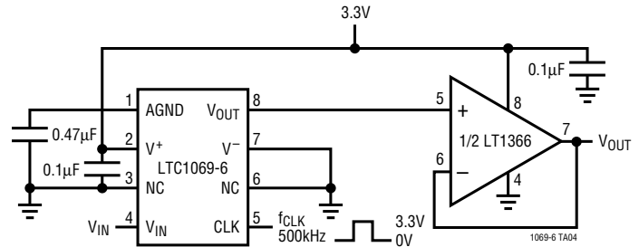
Single 3V Supply Voice Band Lowpass Filter with Rail-to-Rail Input and Output
