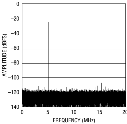
LTC2204: 64K Point FFT, 40Msps, f_{IN} = 5.1\text{MHz} , -25dBFS, PGA = 0, DITH = 0
