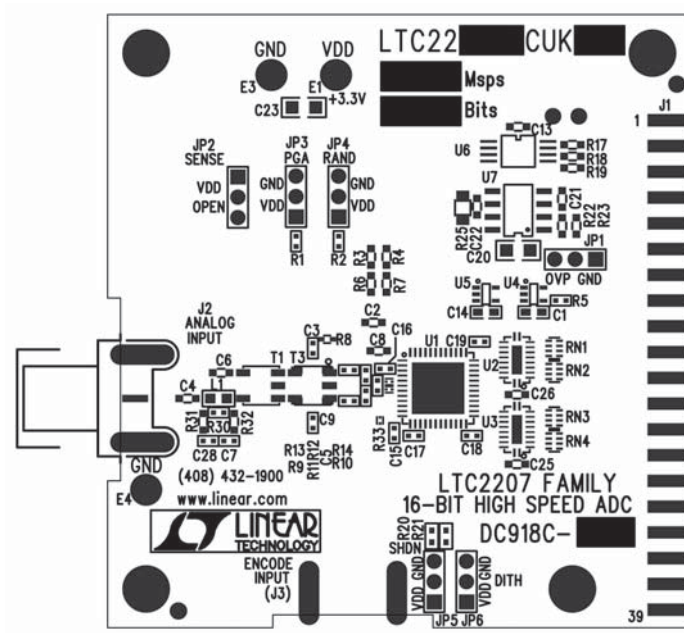
Silkscreen Top
