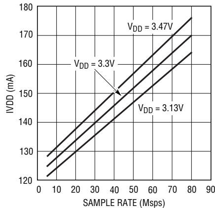
LTC2204: IVDD vs Sample Rate, f_{IN} = 5.1\text{MHz} , 1\text{dBFS} , DITH = 0, RAND = 0
