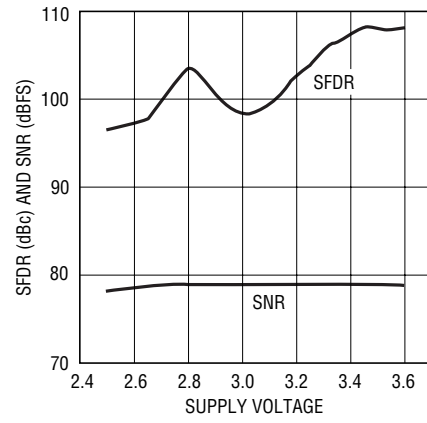
LTC2205: SFDR and SNR vs Supply Voltage, f_{IN} = 5.1\text{MHz} , 65\text{MSPS} , PGA = 0
