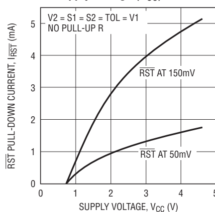
\overline{RST} Pull-Down Current ( I_{RST} ) vs Supply Voltage ( V_{CC} )
