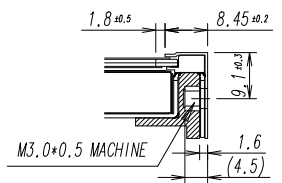
SEC. C-C'
