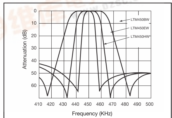
Figure 3) LTM450W – Characteristics
