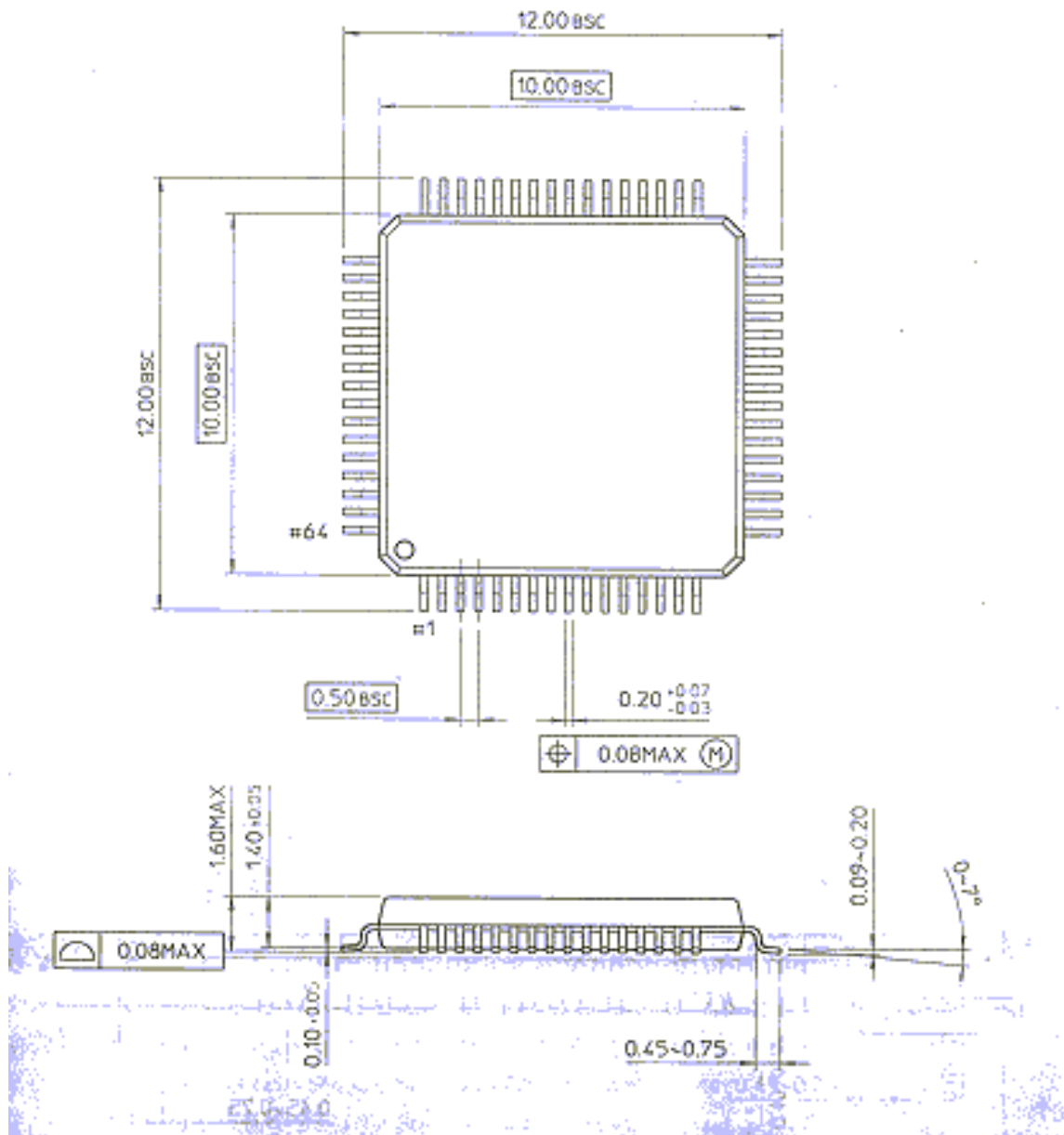
Fig.3 Dimension
