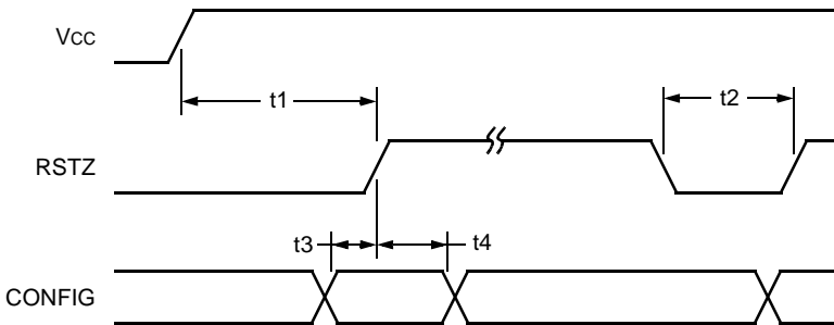
Figure 18. Reset and Configuration Timing
