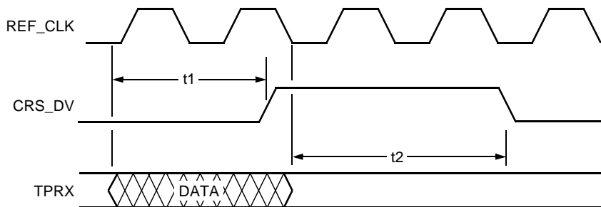
Figure 16. Receive Timing
