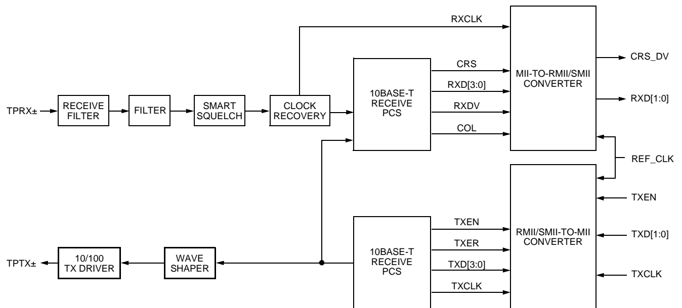
Figure 10. 10Base-T Module Data Path
