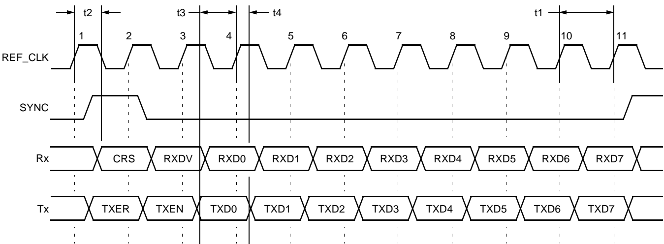
Figure 17. SMII Timing
