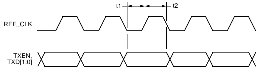
Figure 14. RMII Transmit Timing
