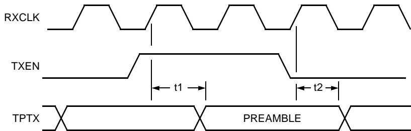
Figure 15. Transmit Timing
