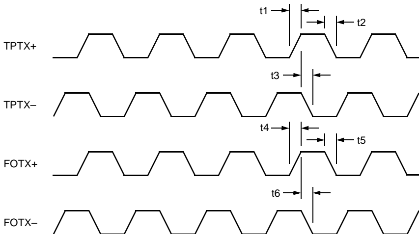
Figure 19. PMD Characteristics
