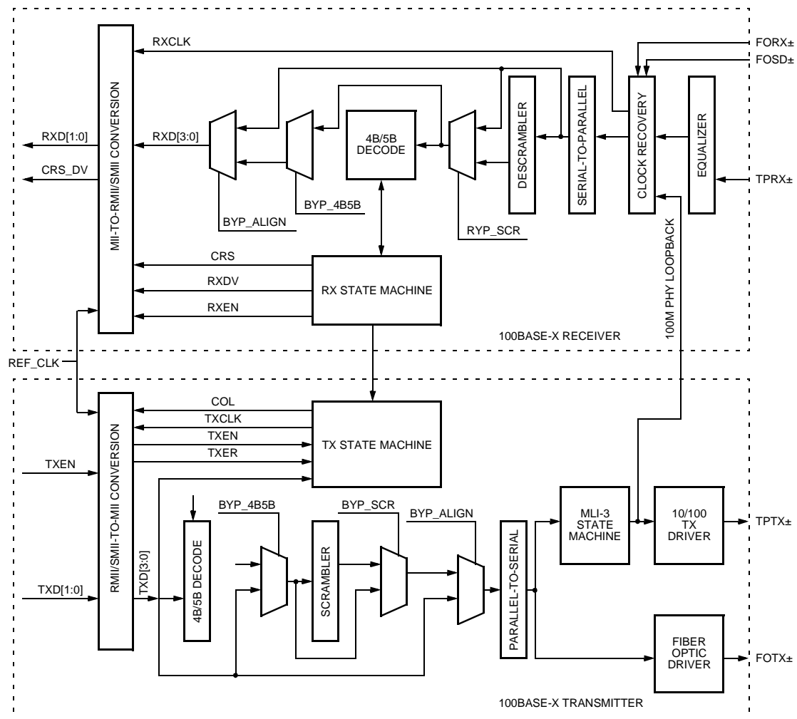
Figure 9. 100Base-X Data Path
