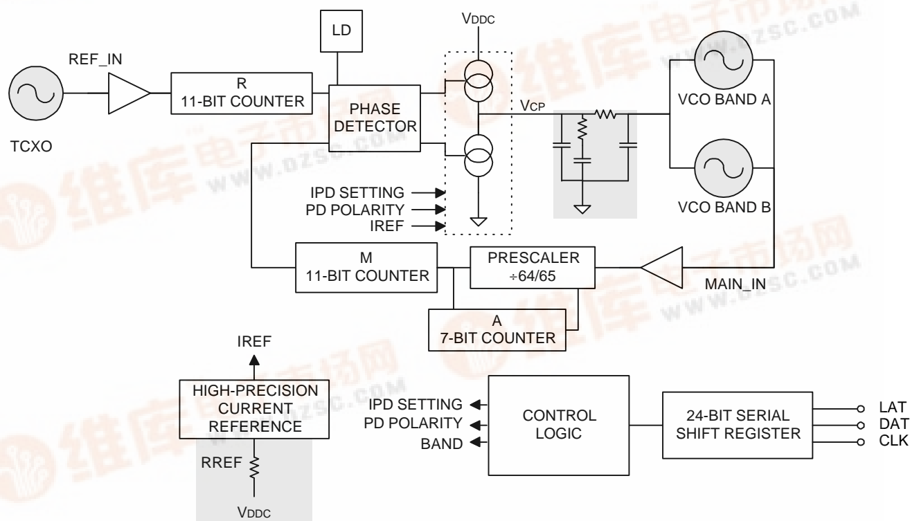
Figure 1. Block Diagram with Pinout
