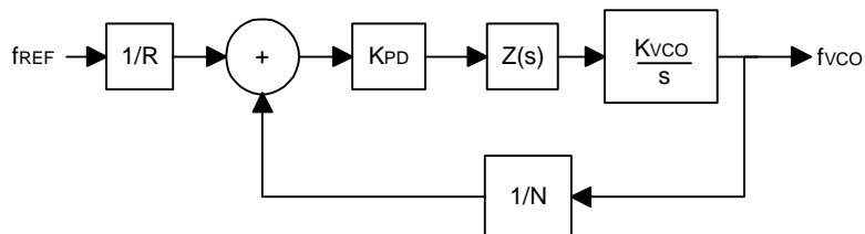
Figure 11. Typical PLL Model
