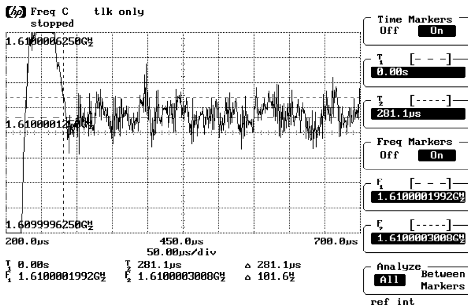
Figure 20. Settling Time from 1150 MHz to 1230 MHz ± 50 Hz
