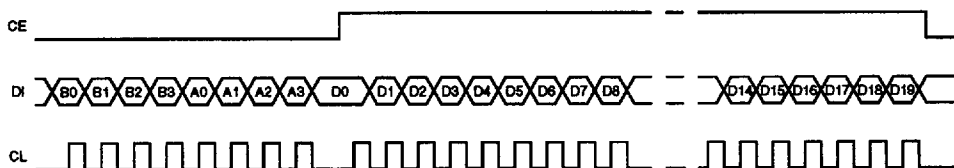
Figure 1. Input timing
