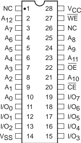
DIP Package (P)
