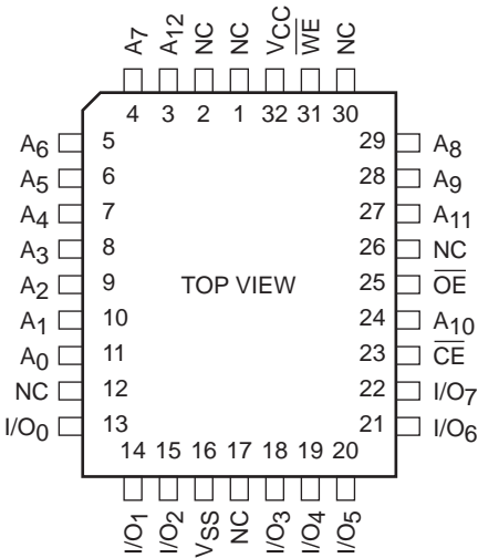
PLCC Package (N)
