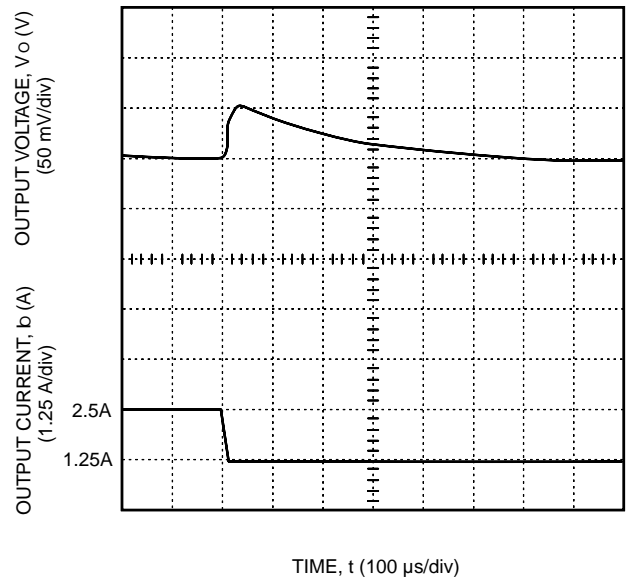
Figure 7. LW025A, F Typical Output Voltage for a Step Load Change from 50% to 25%
