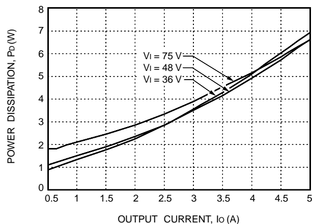
Figure 18. LW025A Power Dissipation vs. Output Current, T_a = 25\text{ }^\circ\text{C}
