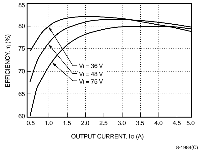
Figure 6. LW025A Typical Converter Efficiency vs. Output Current
