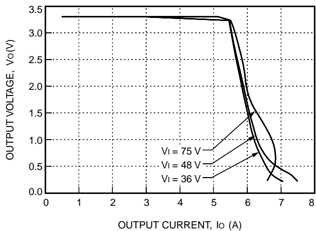
Figure 3. LW025F Typical Output Characteristics
