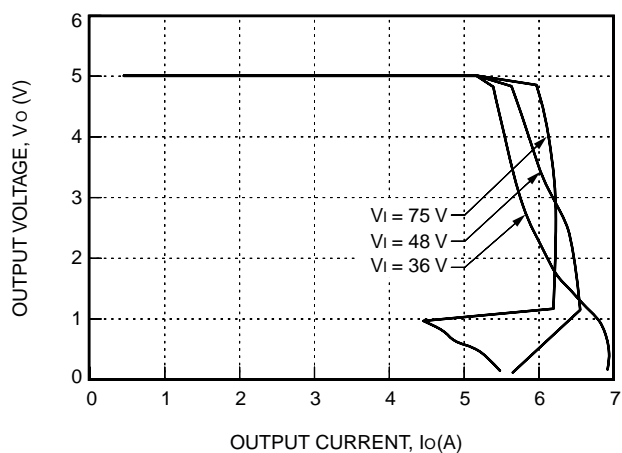
Figure 4. LW025A Typical Output Characteristics
