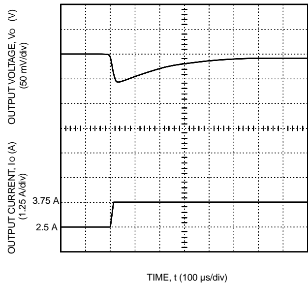
Figure 8. LW025A, F Typical Output Voltage for a Step Load Change from 50% to 75%
