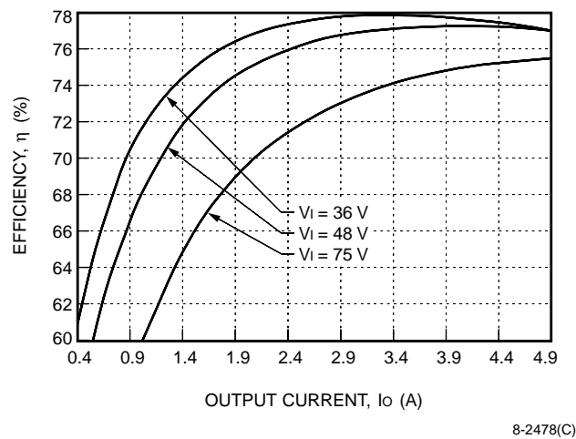
Figure 5. LW025F Typical Converter Efficiency vs. Output Current
