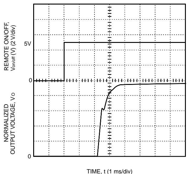
Figure 9. LW025A, F Typical Output Voltage Start-Up when Signal Is Applied to Remote On/Off
