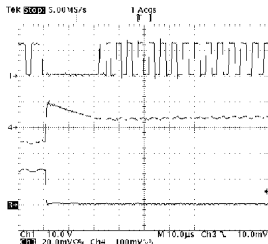
13A Load Transient (in 390ns)
