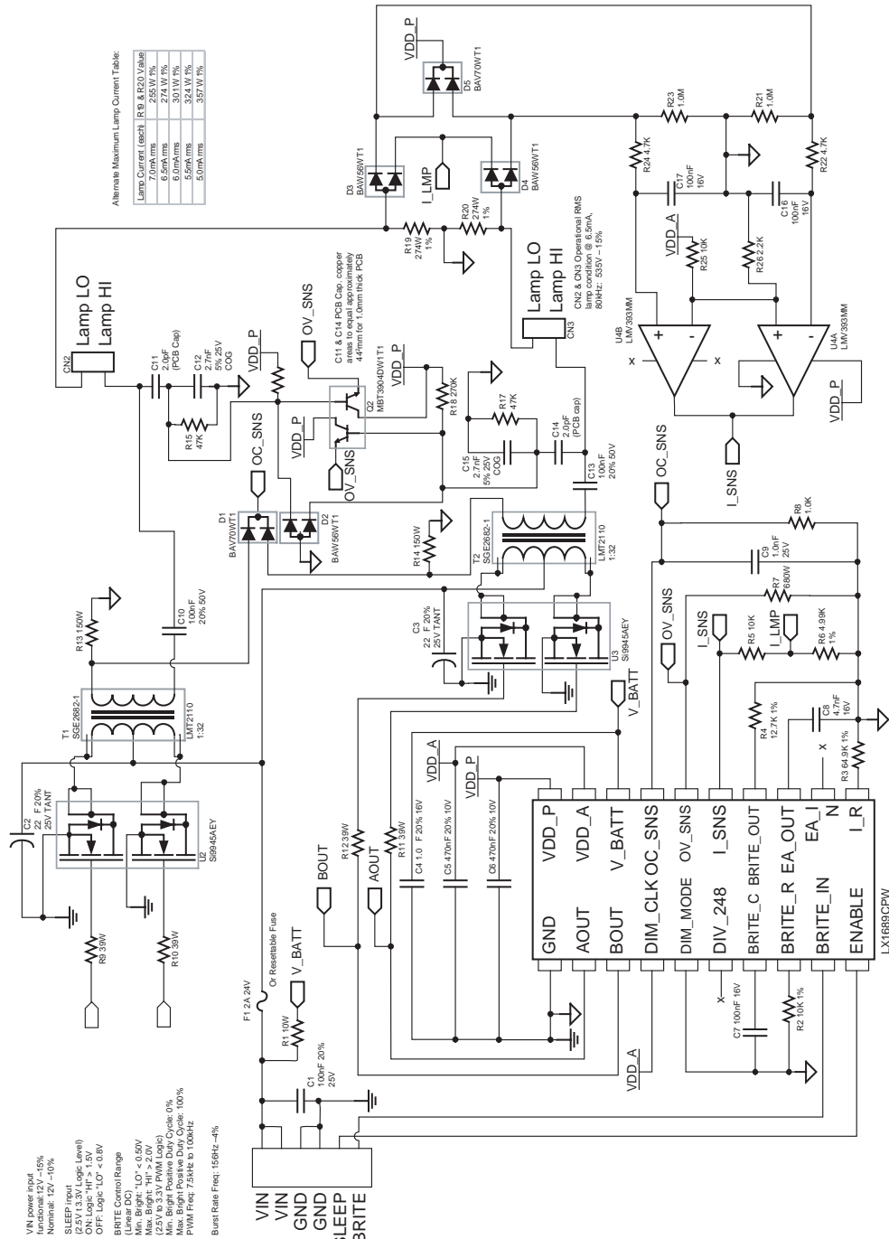
FIGURE 3 – Typical Dual 4 Watt Application
