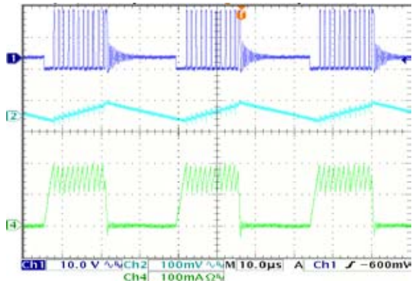
Figure 14 – Typical Switching Waveform
