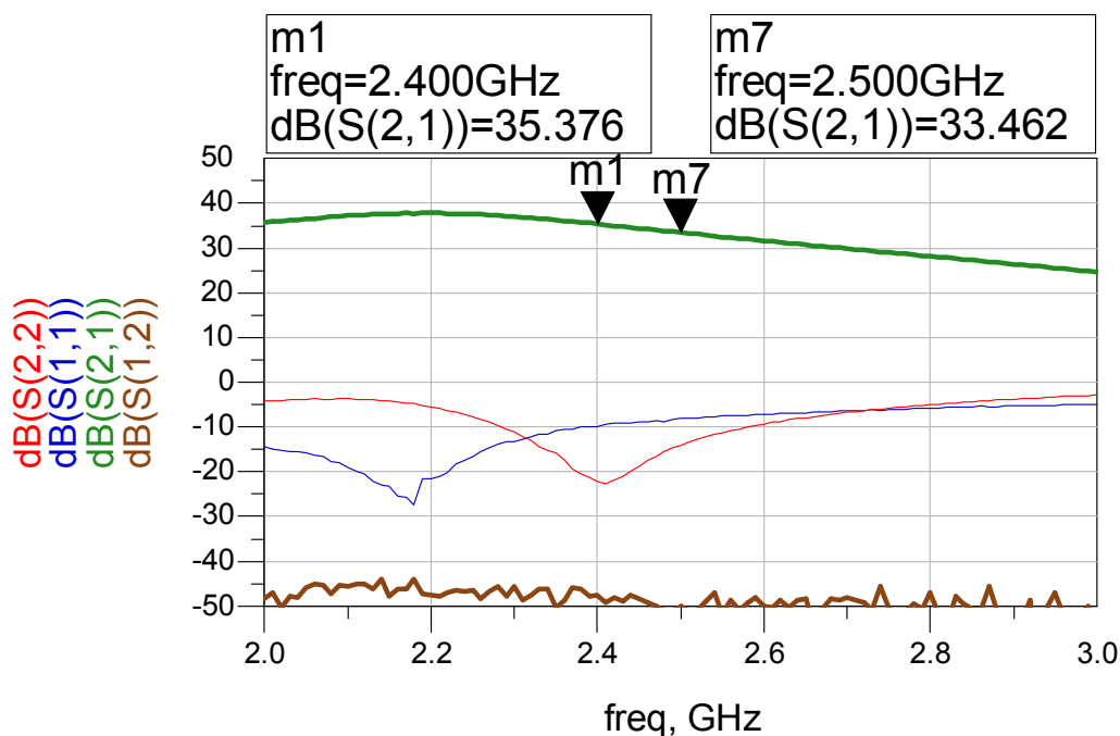
Figure 1 – S-Parameter (VC = 3.3V, VREF = 2.9V, Icq = 50mA)
