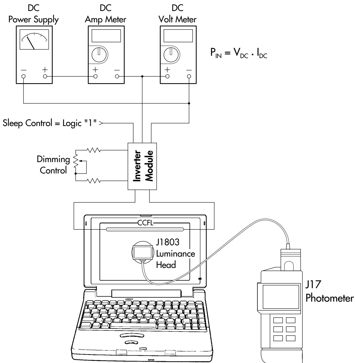
FIGURE 2 — Light Output Measurement Setup
