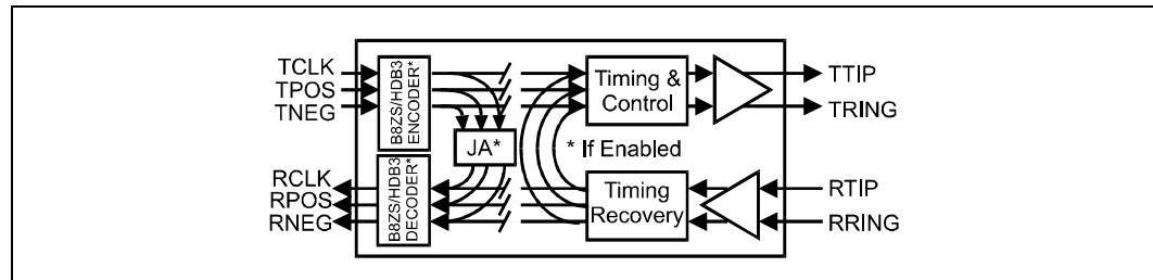
Figure 8. Dual Loopback
