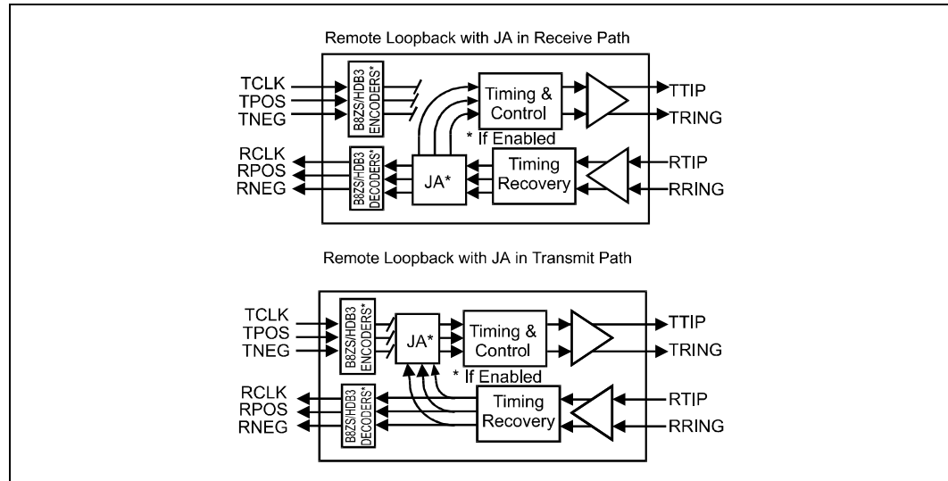
Figure 7. Remote Loopback
