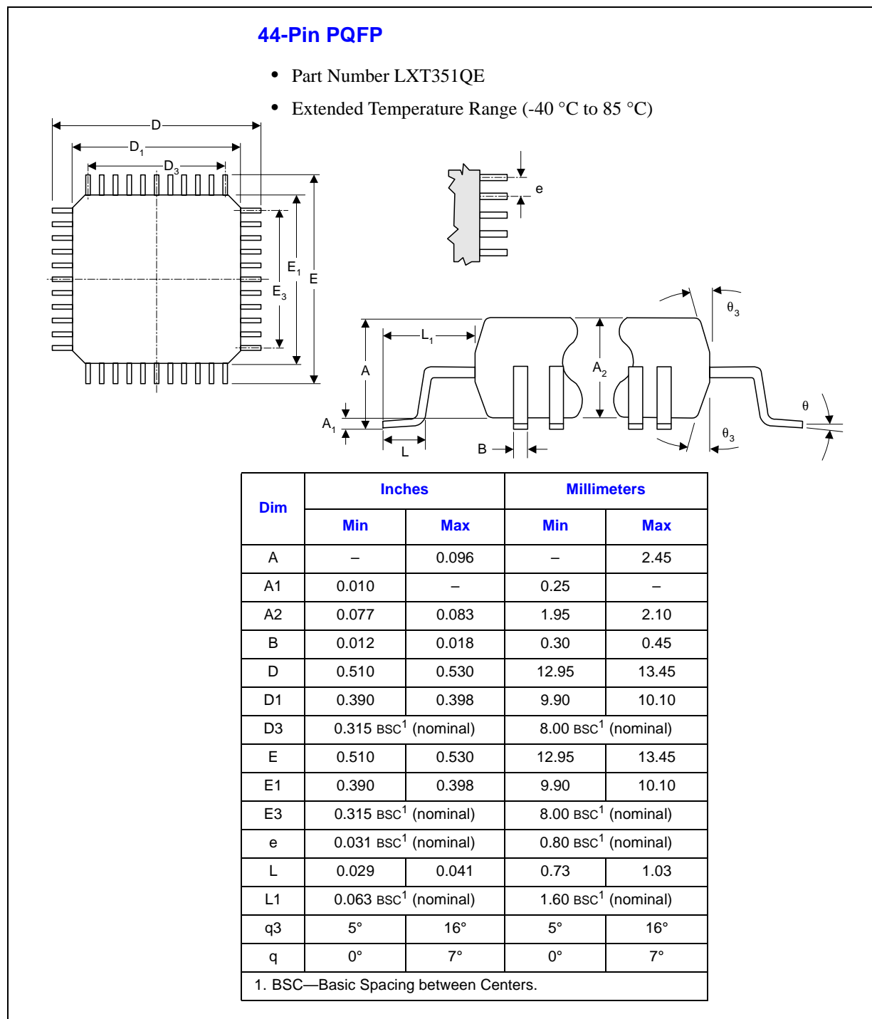
Figure 23. Plastic Quad Flat Package Specifications
