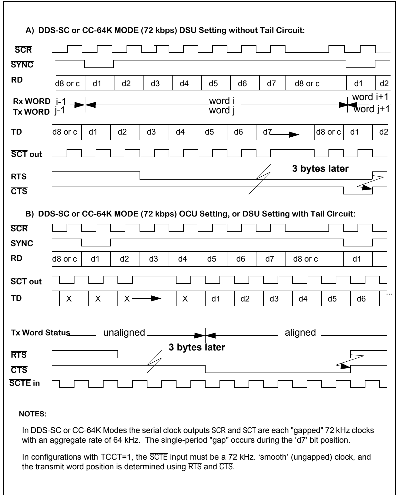
Figure 7: EIA Interface Data Structure & Timing - DDS-SC or CC-64K Mode
