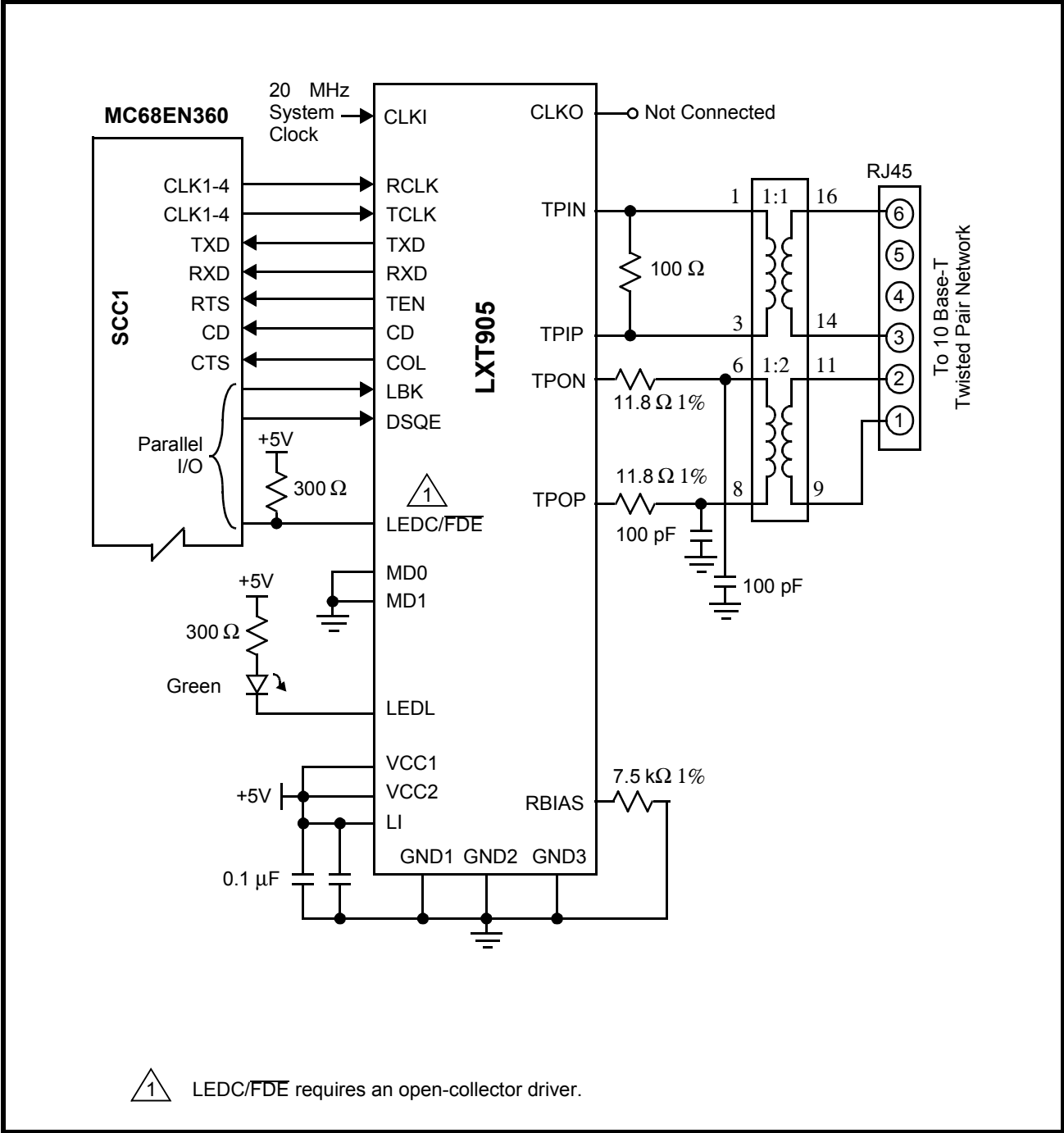
Figure 9: LXT905/MC68EN360 Interface for Full Duplex 10BASE-T (Mode 1)
