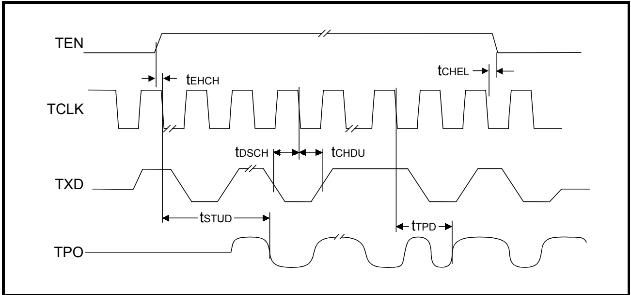
Figure 20: Mode 3 Transmit Timing
