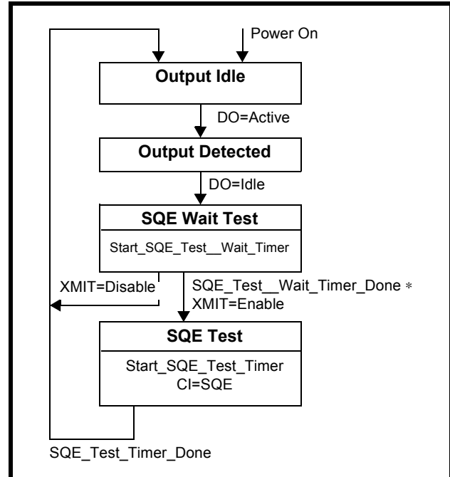
Figure 4: Signal Quality Error (SQE) Function
