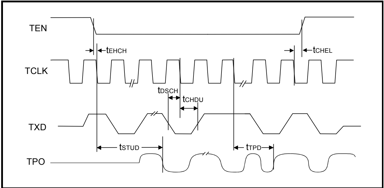
Figure 16: Mode 2 Transmit Timing
