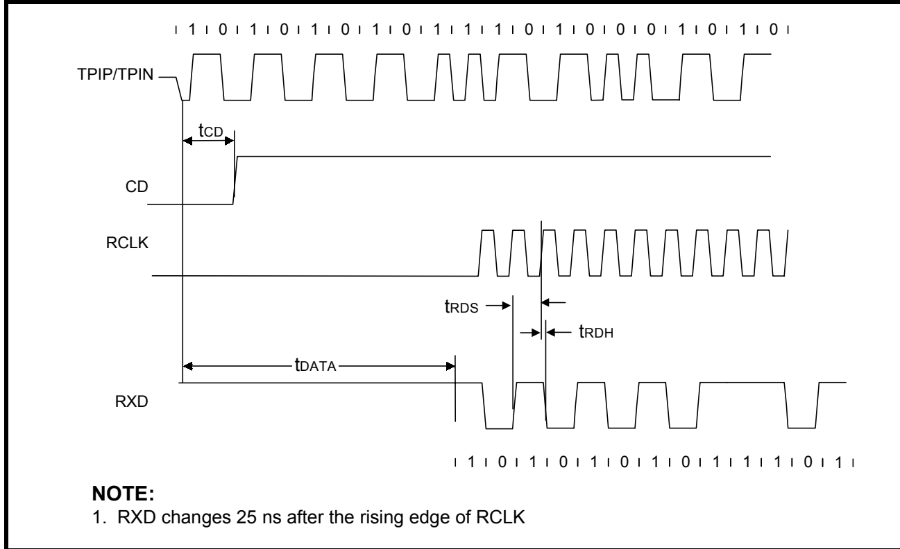
Figure 10: Mode 1 RCLK/Start-of-Frame Timing
