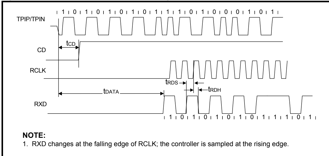
Figure 22: Mode 4 RCLK/Start-of-Frame Timing
