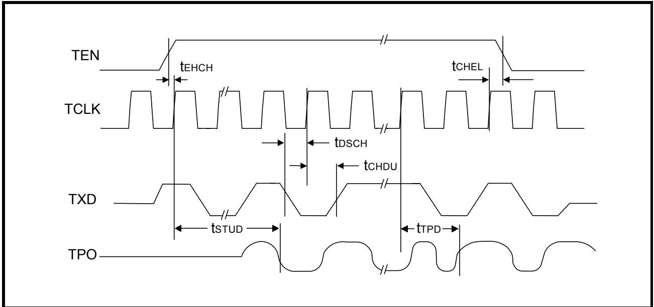
Figure 12: Mode 1 Transmit Timing
