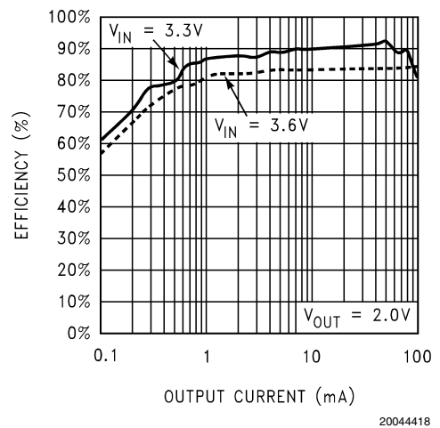
Efficiency vs. Output Current: LM2788-2.0
