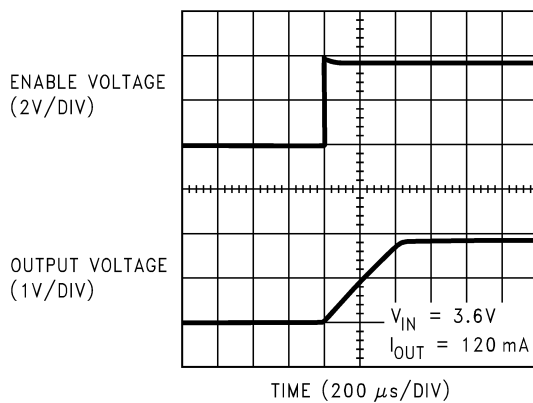
Start Up Waveform
