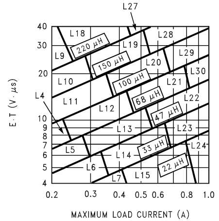
FIGURE 7. LM2672-ADJ
