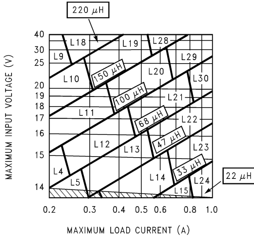
FIGURE 6. LM2672-12
