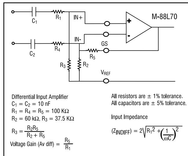
Figure 7 Differential Input Configuration
