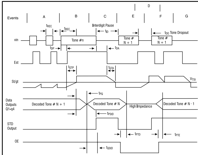
Figure 6 Timing Diagram
