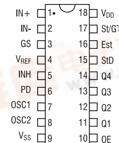
Figure 1 Pin Connections
