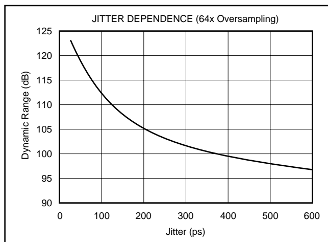
FIGURE 16. Jitter Sensitivity.
