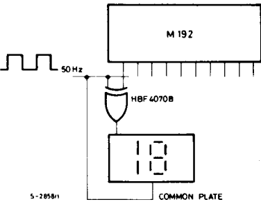
Fig. 2 - Liquid crystal readout
