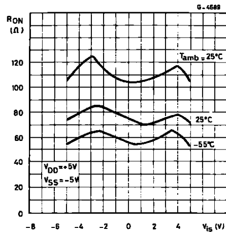
Typical ON Resistance vs. Input Signal Voltage at V_{DD} = -V_{SS} = 5\text{ V} .
