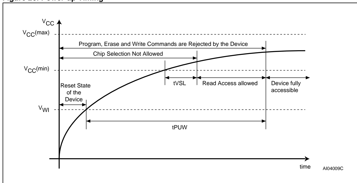
Figure 20. Power-up Timing
