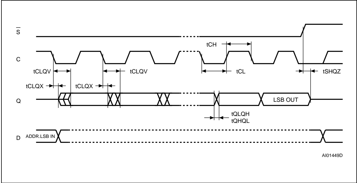
Figure 27. Output Timing
