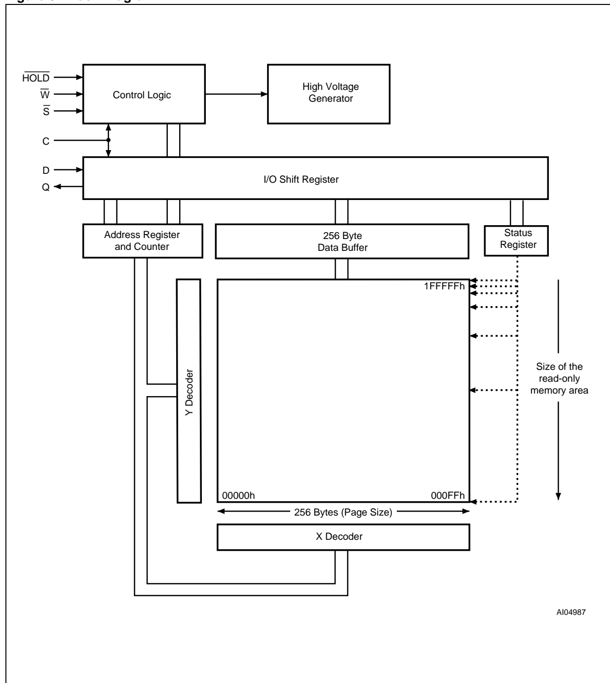
Figure 8. Block Diagram
