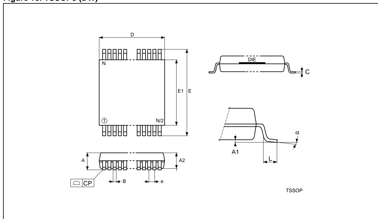
Figure 15. TSSOP8 (DW)
