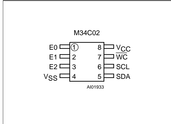
Figure 2B. SO and TSSOP Connections
