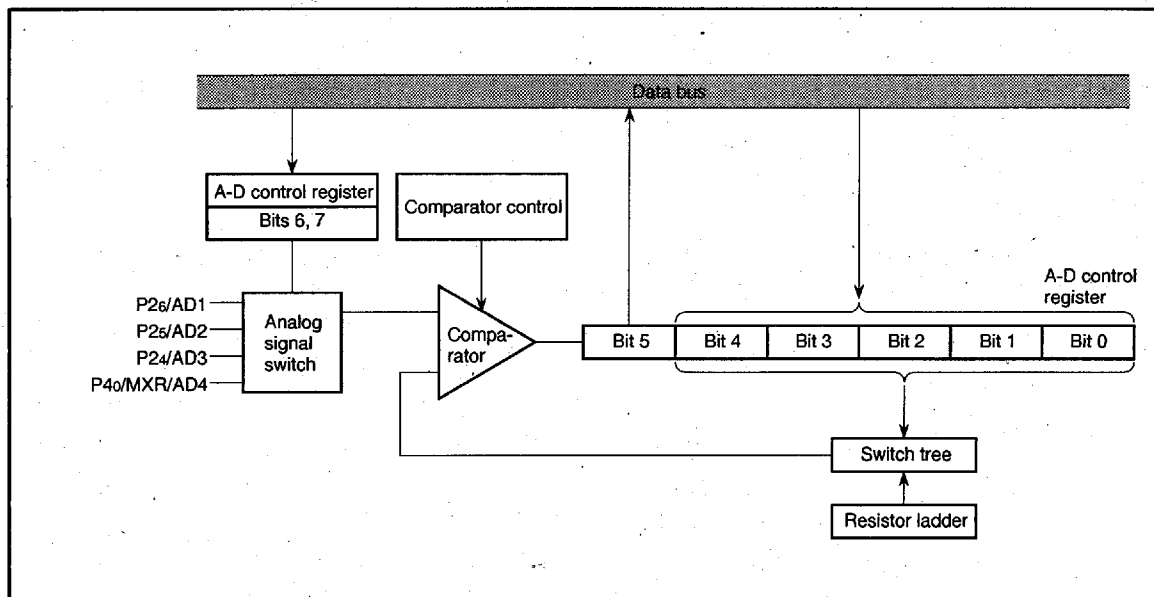
Fig. 15 A-D comparator block diagram
