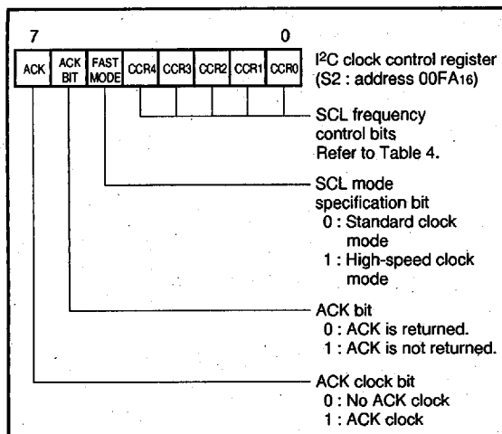
Fig. 35 Structure of I²C clock control register
