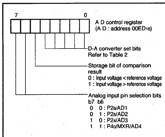
Fig. 16 Structure of A-D control register
