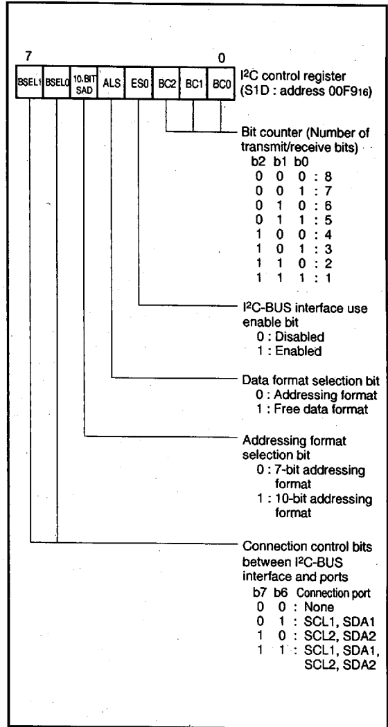
Fig. 37 Structure of I²C control register
