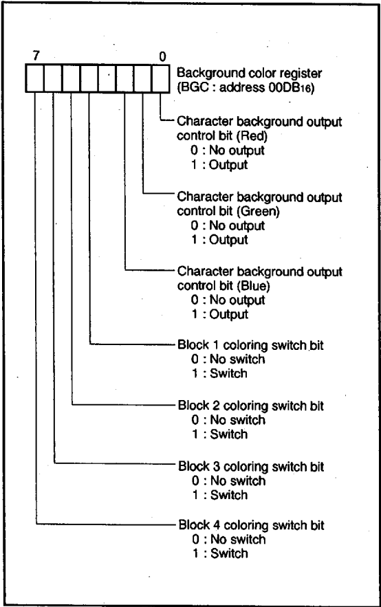
Fig. 65 Structure of background color register
