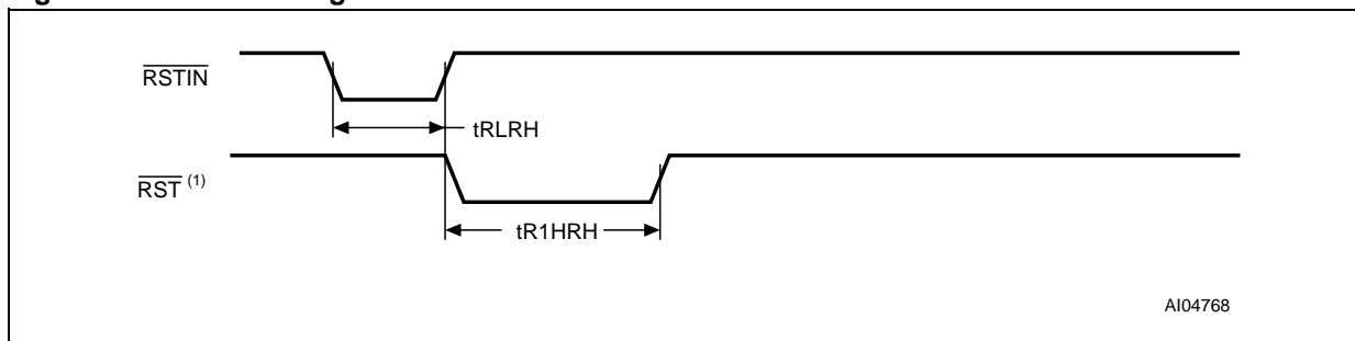
Figure 12. \overline{\text{RSTIN}} Timing Waveform
