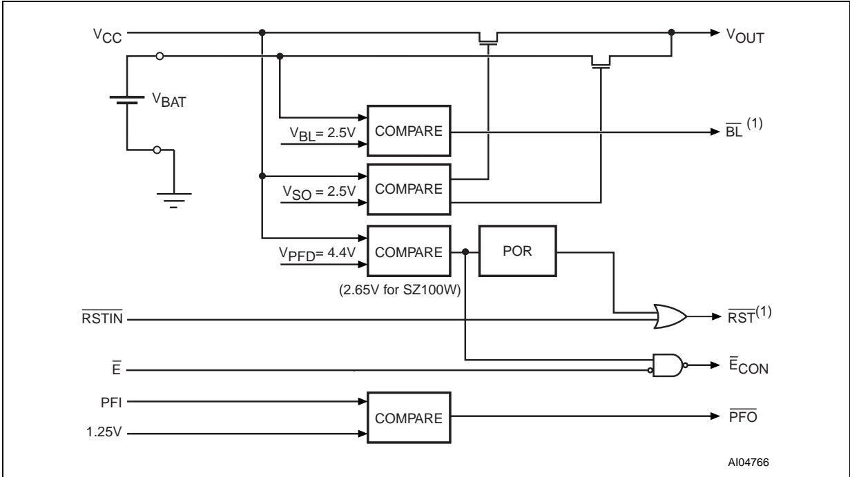
Figure 6. Block Diagram
