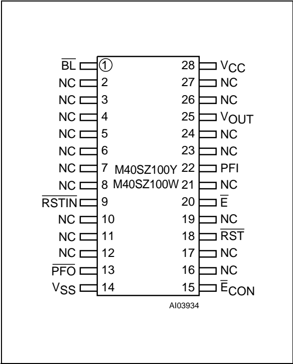
Figure 5. SOIC28 Connections
