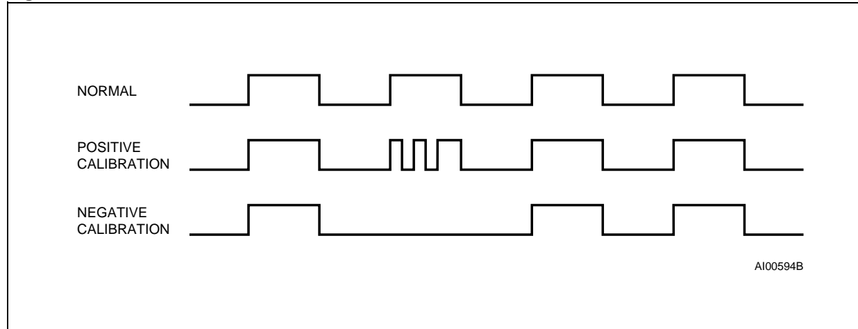
Figure 13. Clock Calibration
