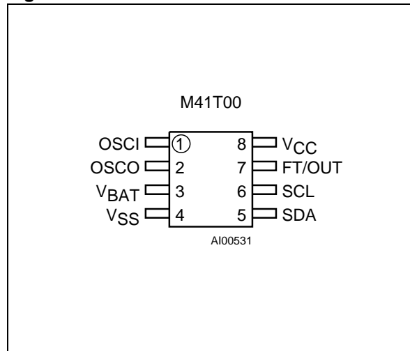
Figure 2. SOIC Connections
