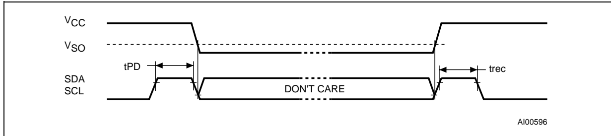
Figure 14. Power Down/Up Mode AC Waveforms
