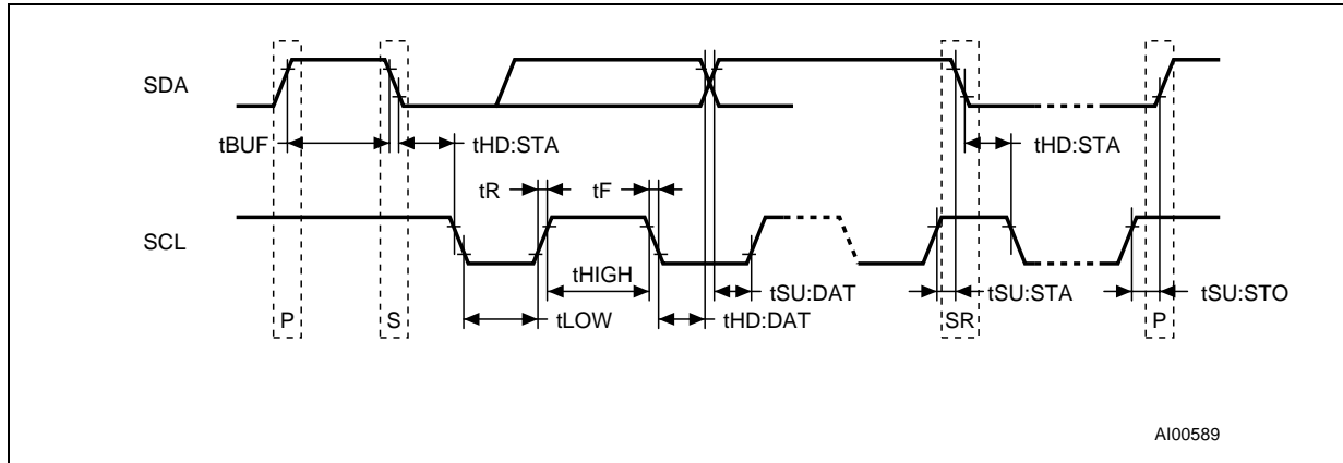
Figure 12. Bus Timing Requirements Sequence
