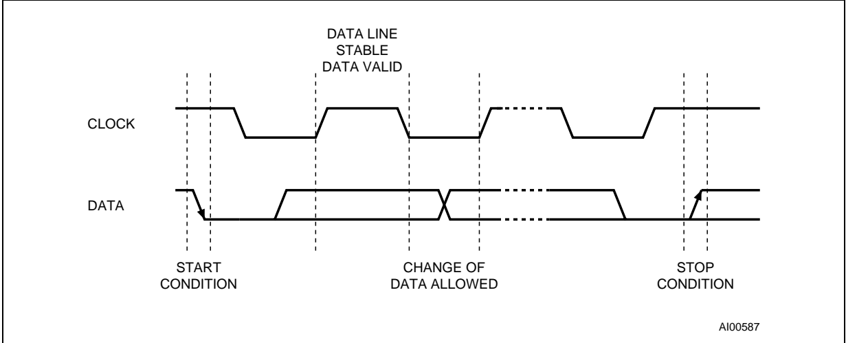
Figure 10. Serial Bus Data Transfer Sequence
