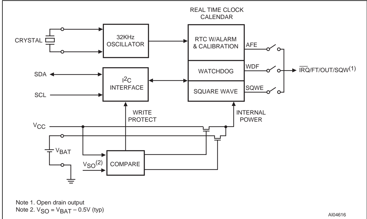
Figure 8. Block Diagram
