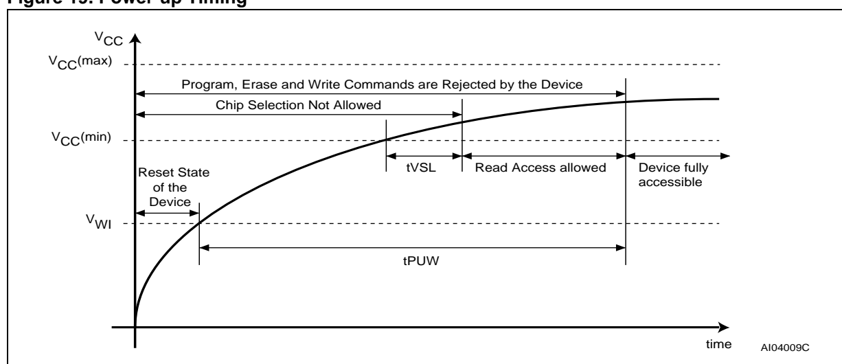
Figure 19. Power-up Timing
