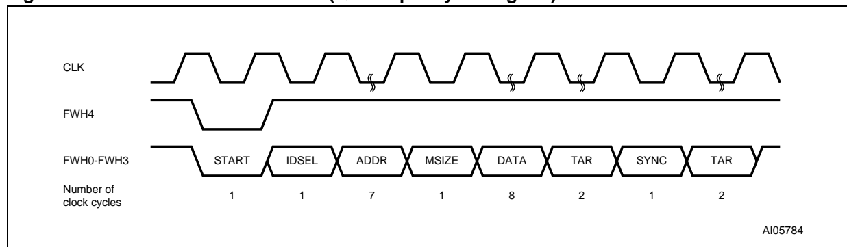
Figure 7. FWH Bus Write Waveforms (Quadruple Byte Program)
