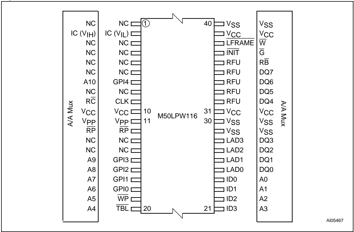
Figure 3. TSOP Connections
