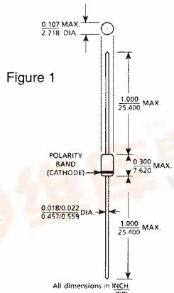
Package Drawing
