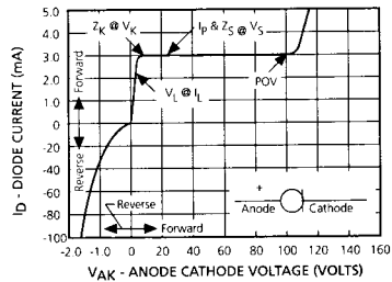
FIGURE 4 Typical Forward Characteristics
