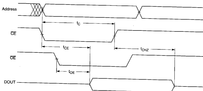
Figure 2. Read Cycle 2
