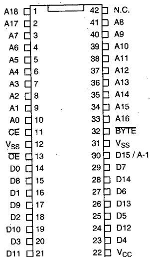
42-Pin DIP
