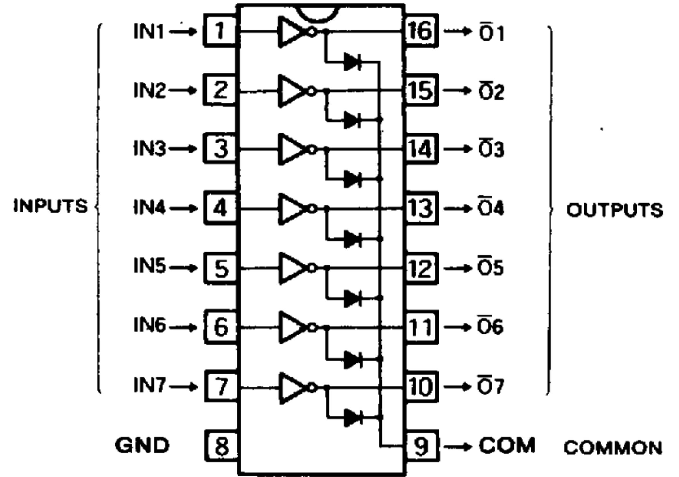
Outline 16P4
