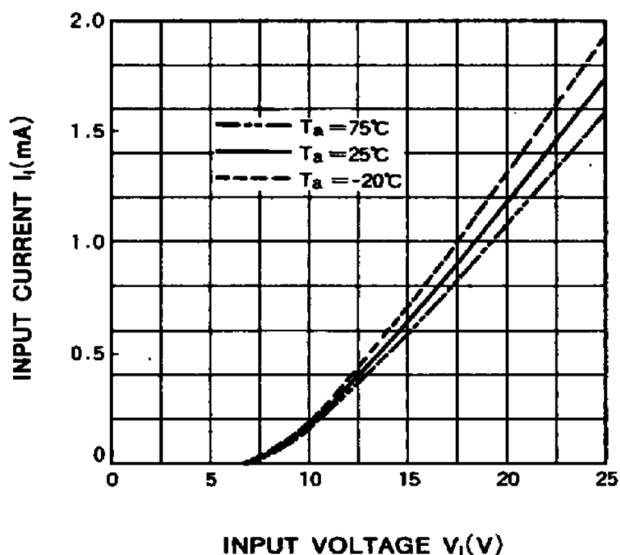
INPUT CHARACTERISTICS
