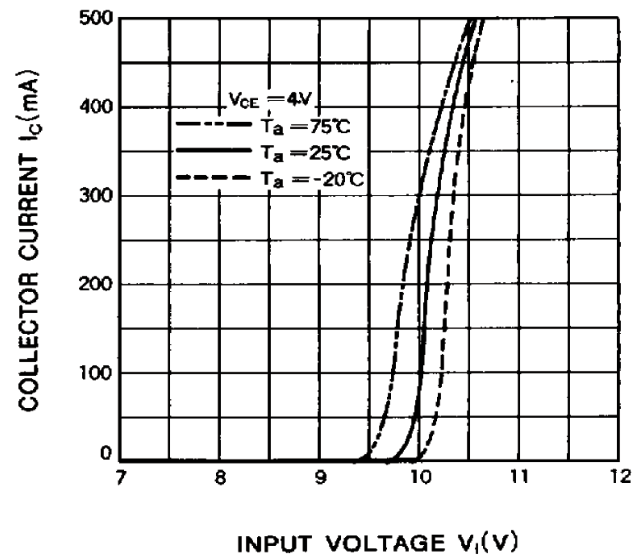
OUTPUT CURRENT CHARACTERISTICS
